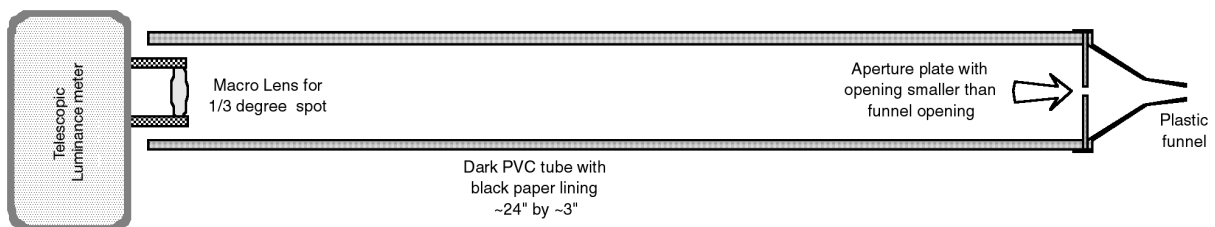
Figure 15. A baffled tube with funnel tip can be used to measure the dark spot in the center of the bright glare pattern. For visual measurements, the same device can be used to view the low-contrast pattern in the dark field. The aperture plate facing the funnel and the funnel exterior and interior should be painted with a nonreflecting black paint.
