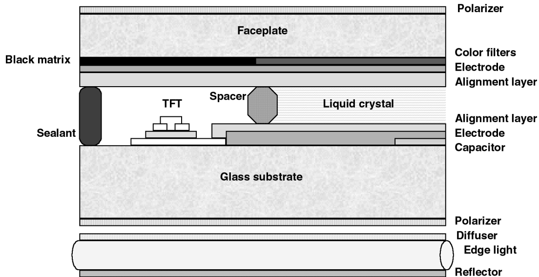
Figure 11. Typical cross section of an AMLCD.
