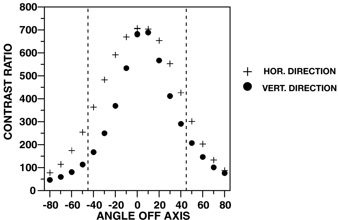
Figure 48. Maximum-to-minimum-luminance contrast ratio of the AMLCD in horizontal and vertical directions. The dashed vertical lines indicate a 90° viewing range ( \pm 45^\circ off-axis) within which the contrast ratio average of the horizontal and vertical directions is always greater than 200 (Blume et al. 2001) (used with permission).
