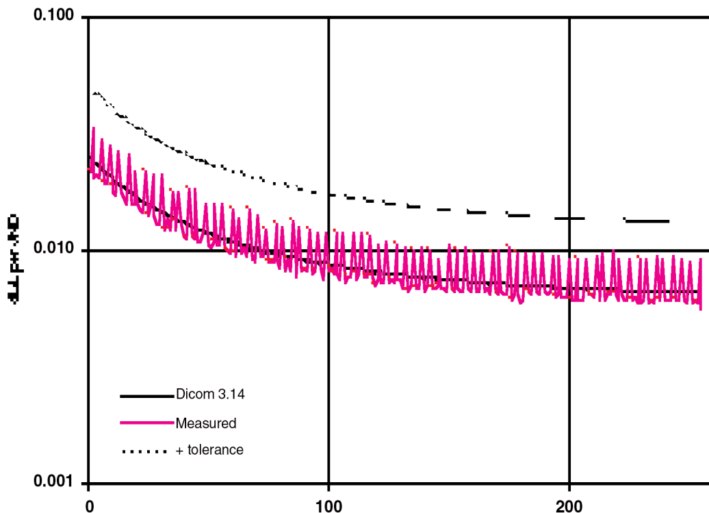
Figure 47. An example of the measured contrast, dL/L , associated with the luminance difference between each of 256 gray levels. The measured contrast has been reduced by the mean number of JND indices per gray level (p-value) and compared to the contrast per JND associated with the DICOM gray scale display function. The results characterize a monochrome LCD display having a luminance calibration derived from a set of 766 possible luminance values.
