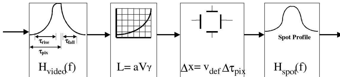
Figure 8. Model of a CRT display device, illustrating components affecting its spatial resolution: (a) response function of video circuits of display controller and CRT display device; (b) the non-linear relationship between the luminance and the input voltage; (c) the scanning speed of the deflection unit; and (d) the finite size and shape of the focal spot.
