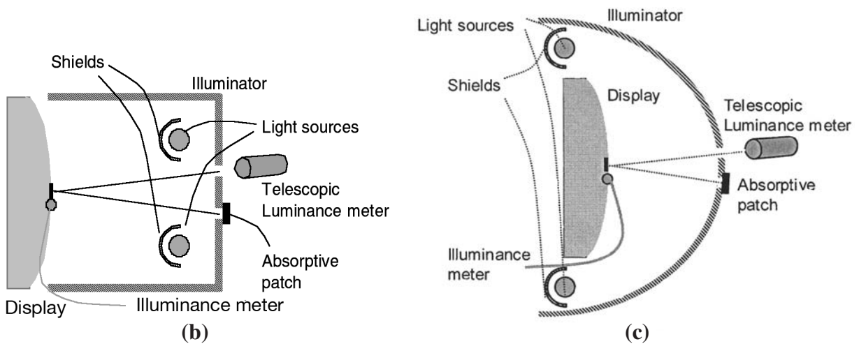
Figure 19. A typical illuminating device used for quantitative measurements of the diffuse reflection of a display device (a). The lamps should ideally be baffled from directly illuminating the display surface (b) or otherwise be placed behind the plane of the display illuminating the interior of a semi-hemispherical illumination containment (c).
